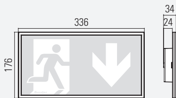
R32W WANDMONTAGE
